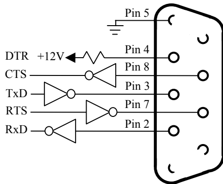
Serial DB9 Male Connector
