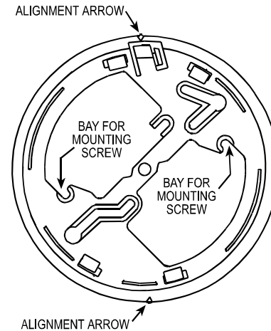
Figure 9. Mounting Bracket
