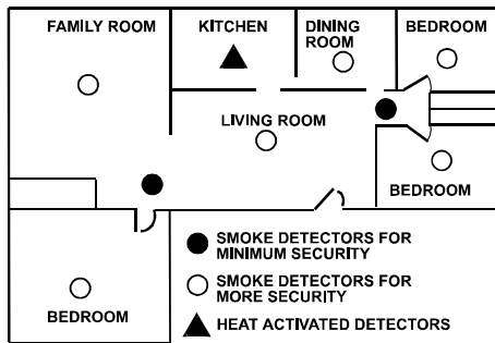
Figure 4. Placement of Smoke/Heat Detectors in Single-Floor Residence with More than One Sleeping Area
