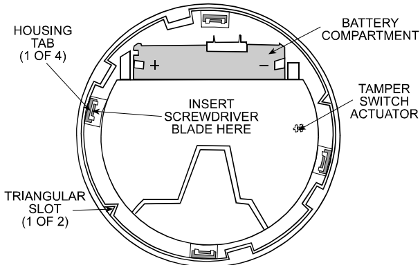
Figure 10. Housing Removal
