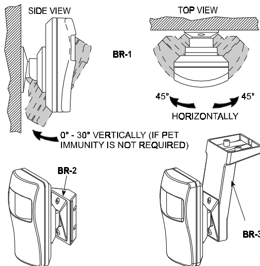
Figure 5. Optional Swivel Brackets
