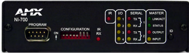
FIG. 1 NI-700 NetLinX Integrated Controller (front view)
