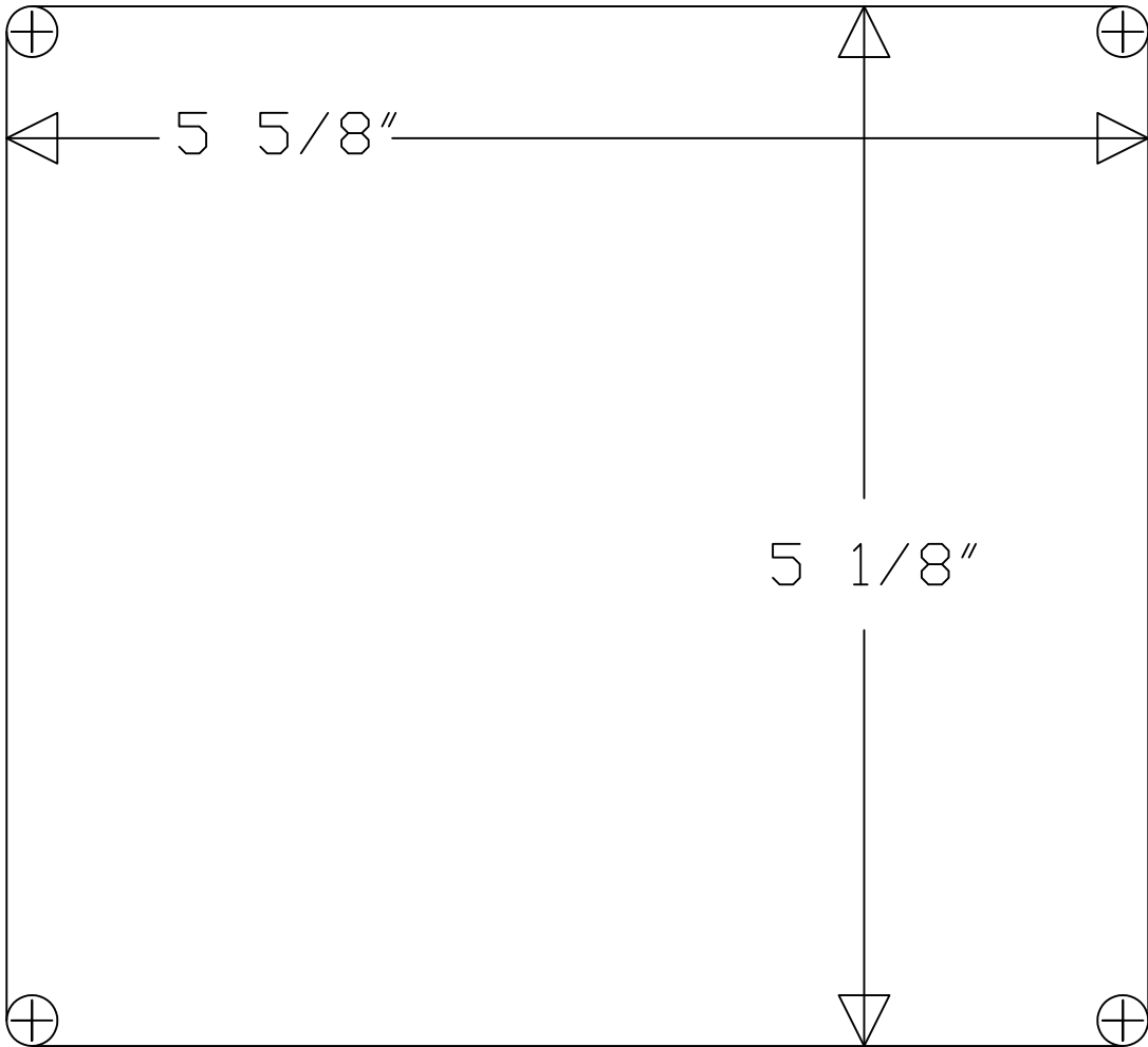
Installation Template - 53A10-1
